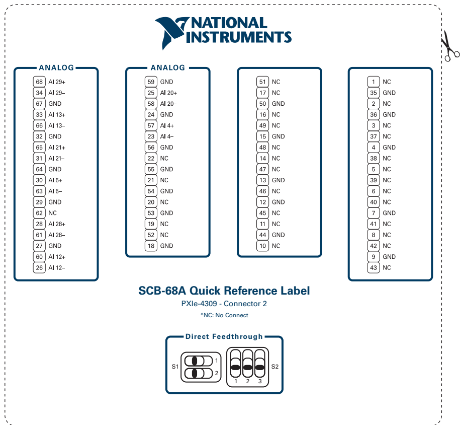
Figure 3. PXIe-4309 Connector 2
