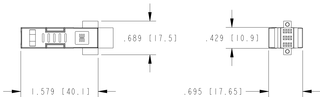
BACKSHELL WITH 6 POS CONNECTOR
