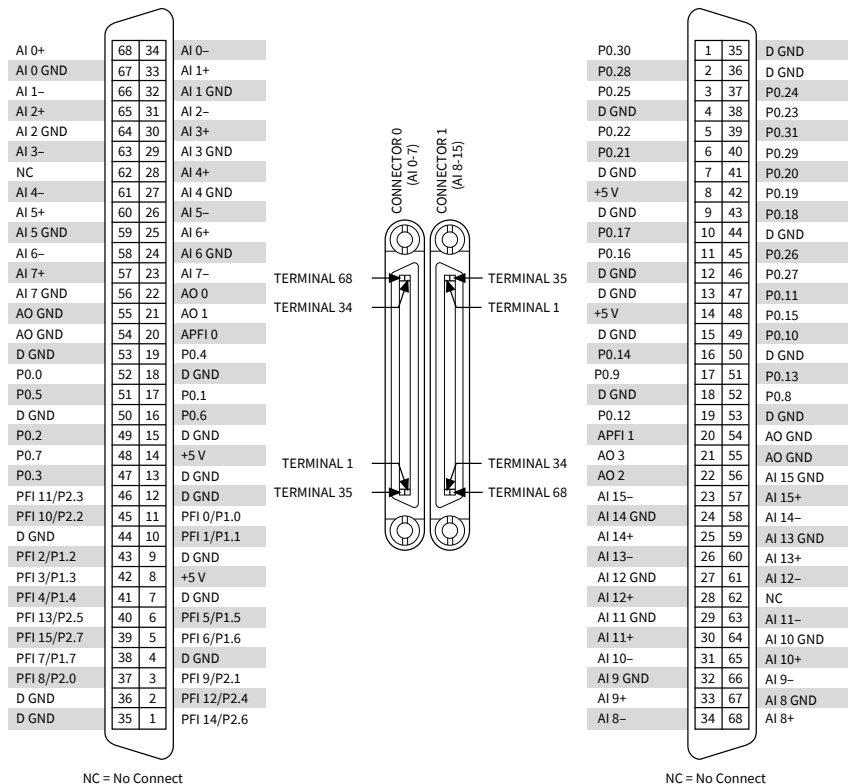
Figure 6. NI PXle-6358 Pinout
