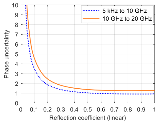
Measured uncertainty of reflection magnitude and reflection phase measurements for the R&S® ZNL 1 ; analysis conditions: S_{12} = S_{21} = 0 , calibrated power -10 dBm, measured power -10 dBm
