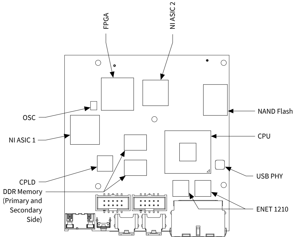
Figure 2. sbRIO-9609 Component Locations
