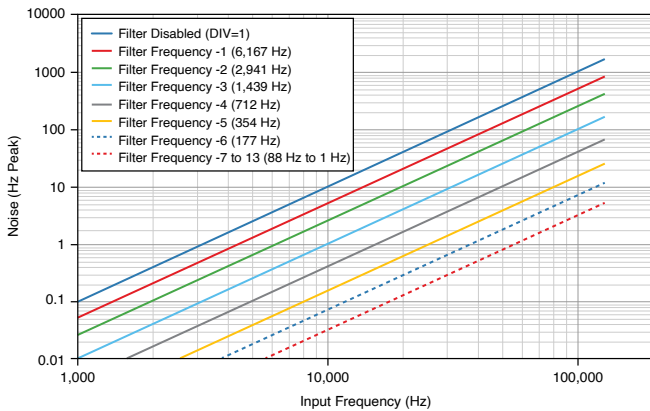
Figure 2. Frequency Noise
