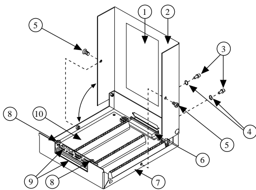
Figure 1. SCB-68 Parts Locator Diagram
