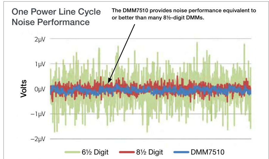
Comparison of the DMM7510's 1 VDC noise performance with that of typical 6½- and 8½-digit multimeters. All data was taken at 1 NPLC with a low thermal short applied to the input.
