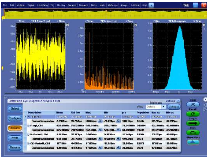
Jitter analysis - TIE jitter/timing analysis of 622 Mb/s signal
