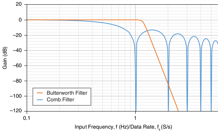
Figure 10. Comparing Typical Magnitude Response of NI 9252 Filters
