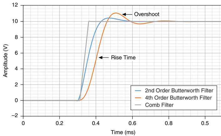
Figure 11. Comparing Typical Step Response of NI 9252 Filters
