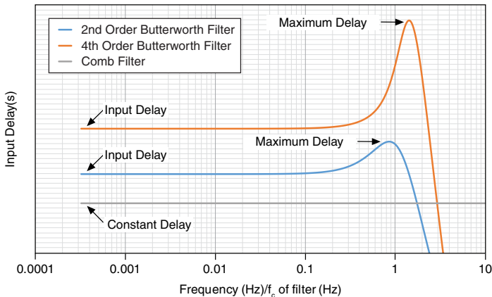
Figure 9. Comparing Typical Input Delay for NI 9252 Filters
