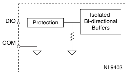
Figure 1. NI 9403 Circuitry
