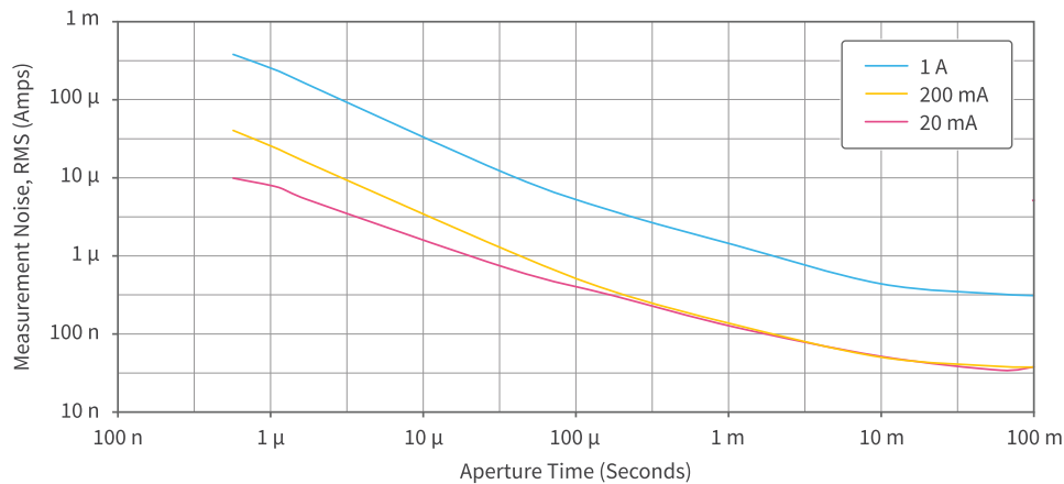
Figure 3. PXIe-4082 DC Current Noise, Typical
