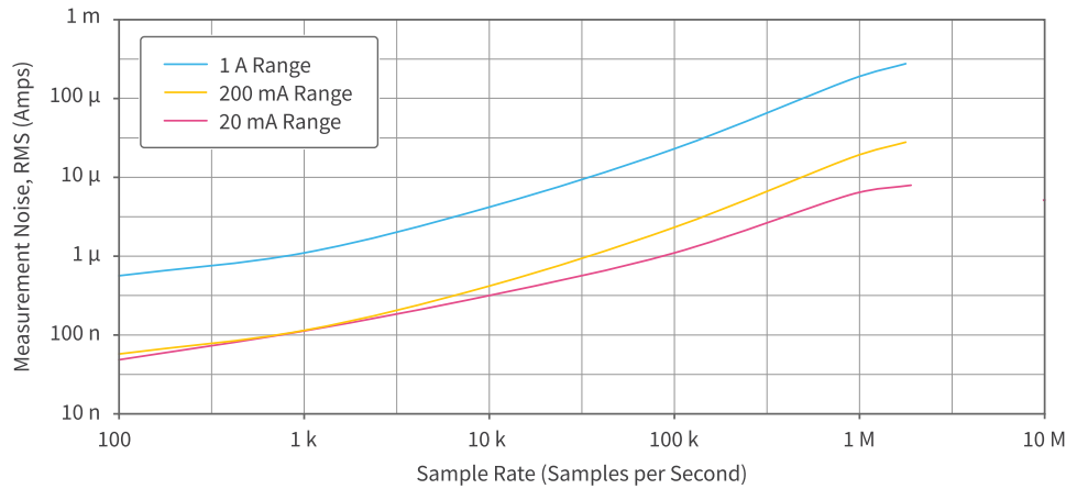
Figure 5. PXIe-4082 Current Waveform Noise with Input Open, Typical
