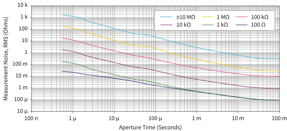
Figure 2. PXIe-4082 Resistance Noise, Typical
