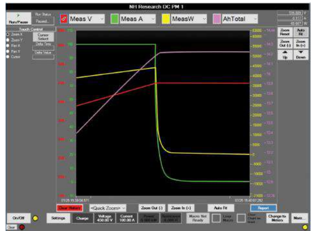
Figure 3 - Chart Recorder
